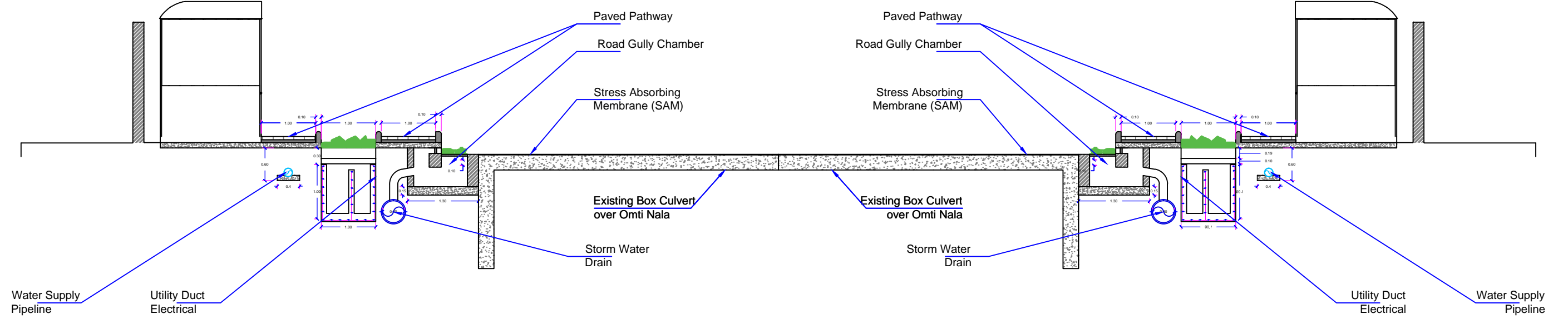
Typical Cross Section NMT
